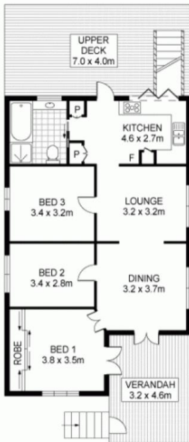
UPPER LEVEL
